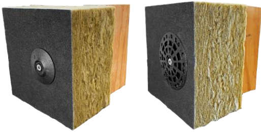
TRUFAST® Walls
