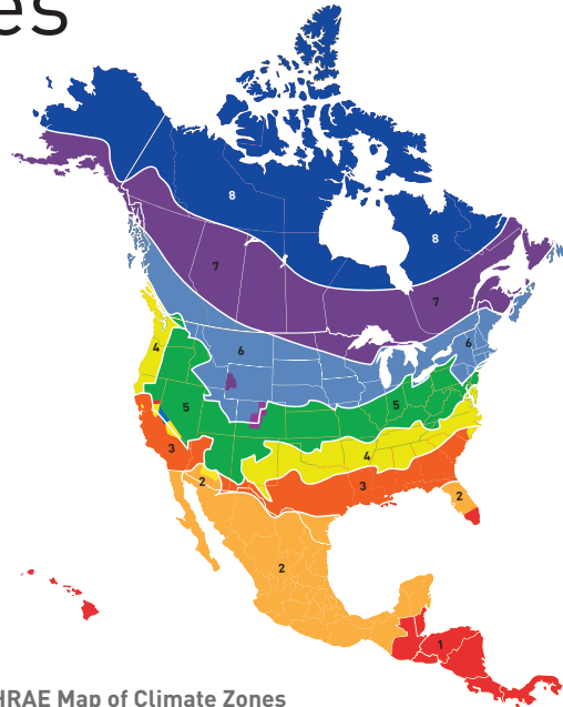
ASHRAE Map of Climate Zones
